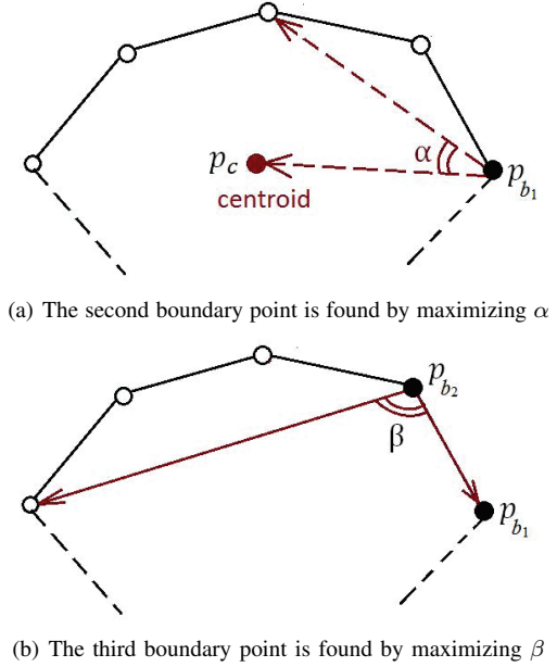
Fig. 5. The Process of finding the boundary points. (a) The first boundary point is chosen as the rightmost point. The second boundary point is found by maximizing \alpha . (b) The third boundary points is found by maximizing \beta . This process is repeated until the first boundary point is encountered again.
