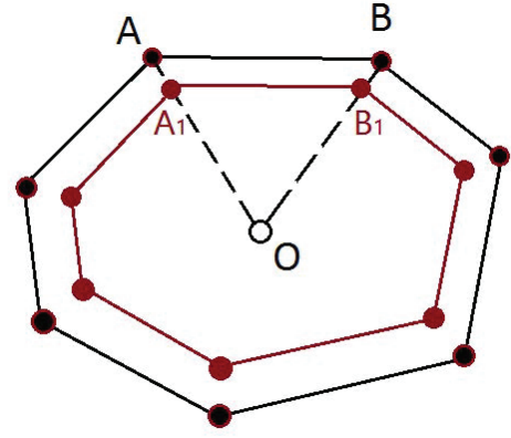
Fig. 7. The shrinking process for a convex hull. Choose an arbitrary point O inside the convex hull, and split the convex hull into a set of triangles (e.g. \triangle OAB ) with the boundaries (e.g. AB ). Shrink each triangle \triangle OAB into a similar triangle \triangle OA_1B_1 . Then the original convex hull (the black one) is shrunk into a smaller convex hull (the red one).
