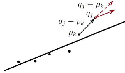
Fig. 4. The velocity of headlamp \mathbf{q}_j (the red arrow) is estimated based on the previous matching result \mathbf{q}_j - \mathbf{p}_k (the dashed arrow) and the average motion direction of all tracked points for this headlamp (the black line).
